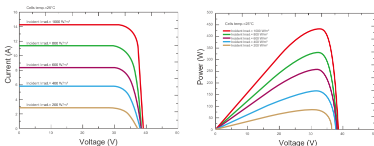
Current-Voltage & Power-Voltage Curves
